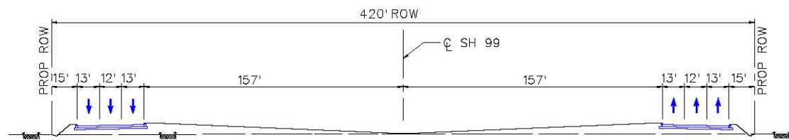
SECTION A-A PHASE 1
